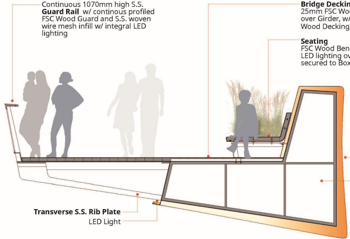
C-C / TRANSVERSE SECTION
